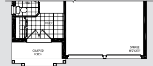
GROUND FLOOR PLAN EL. 'B'
