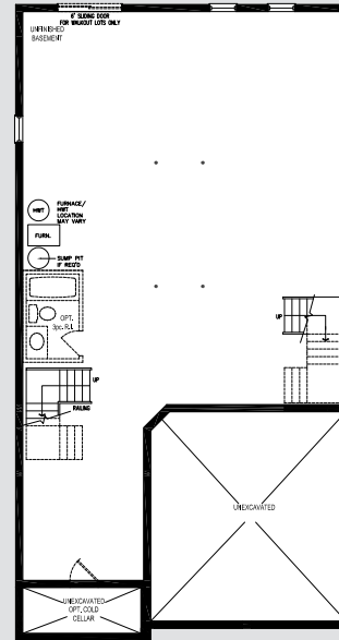
BASEMENT PLAN EL. 'A'
