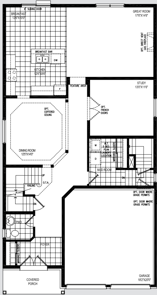
GROUND FLOOR PLAN EL. 'A'
