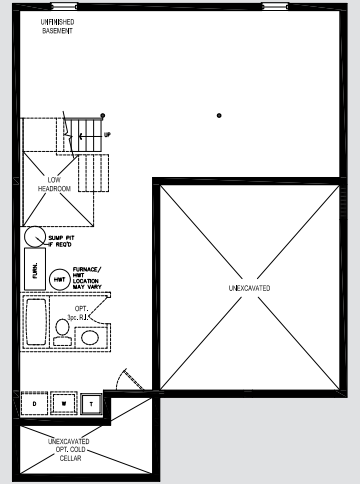
BASEMENT FLOOR PLAN EL. 'A', 'B' & 'C'
