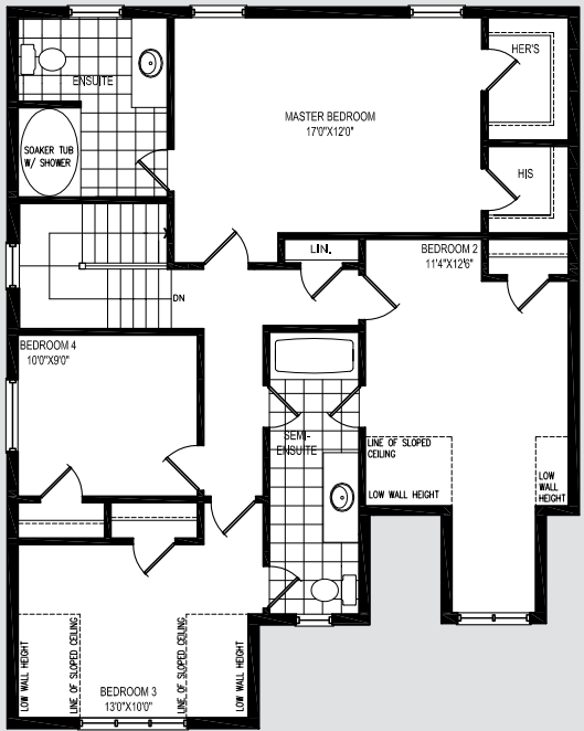
SECOND FLOOR PLAN EL. 'A'
