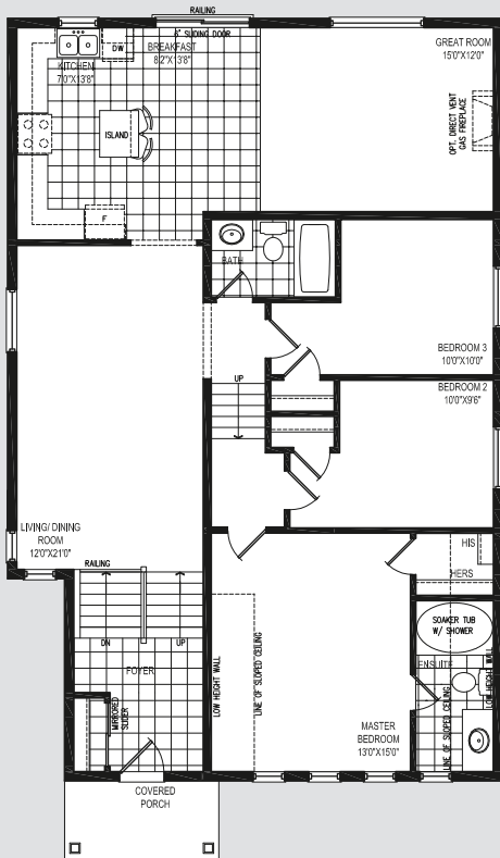
GROUND FLOOR PLAN EL. 'A'
