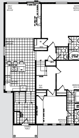
ALT. GROUND FLOOR PLAN EL. 'A'
