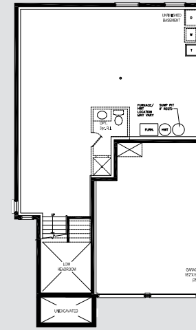
BASEMENT PLAN EL. 'A' & 'C'
